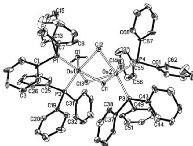
Figure 3. Molecular structure of [(\text{PPh}_3)_2\text{ClOs}(\mu\text{-Cl})_3\text{Os}(\text{H}_2\text{O})(\text{PPh}_3)_2] ( 4 ).
