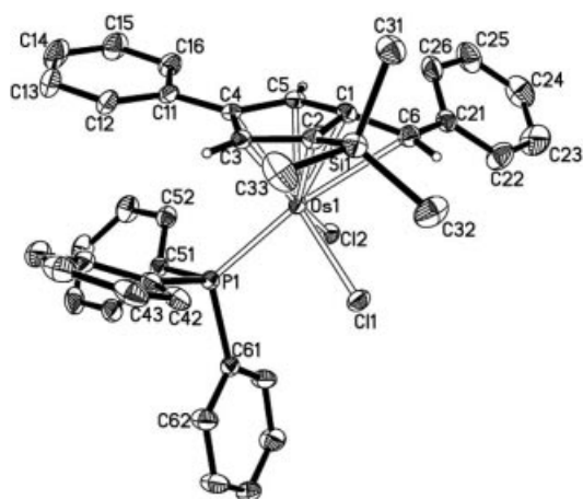
Figure 1. Molecular structure of [\text{OsCl}_2\{\eta^6\text{-C}_5\text{H}_2(\text{Ph})(\text{SiMe}_3)(=\text{CHPh})\}(\text{PPh}_3)] ( 2a ).
