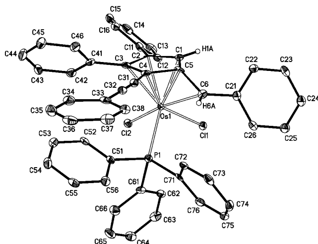
Figure 2. Molecular structure of [\text{OsCl}_2\{\eta^6\text{-C}_5\text{H}(\text{C}\equiv\text{CPh})(\text{Ph})_2(=\text{CHPh})\}(\text{PPh}_3)] ( 3 ).
